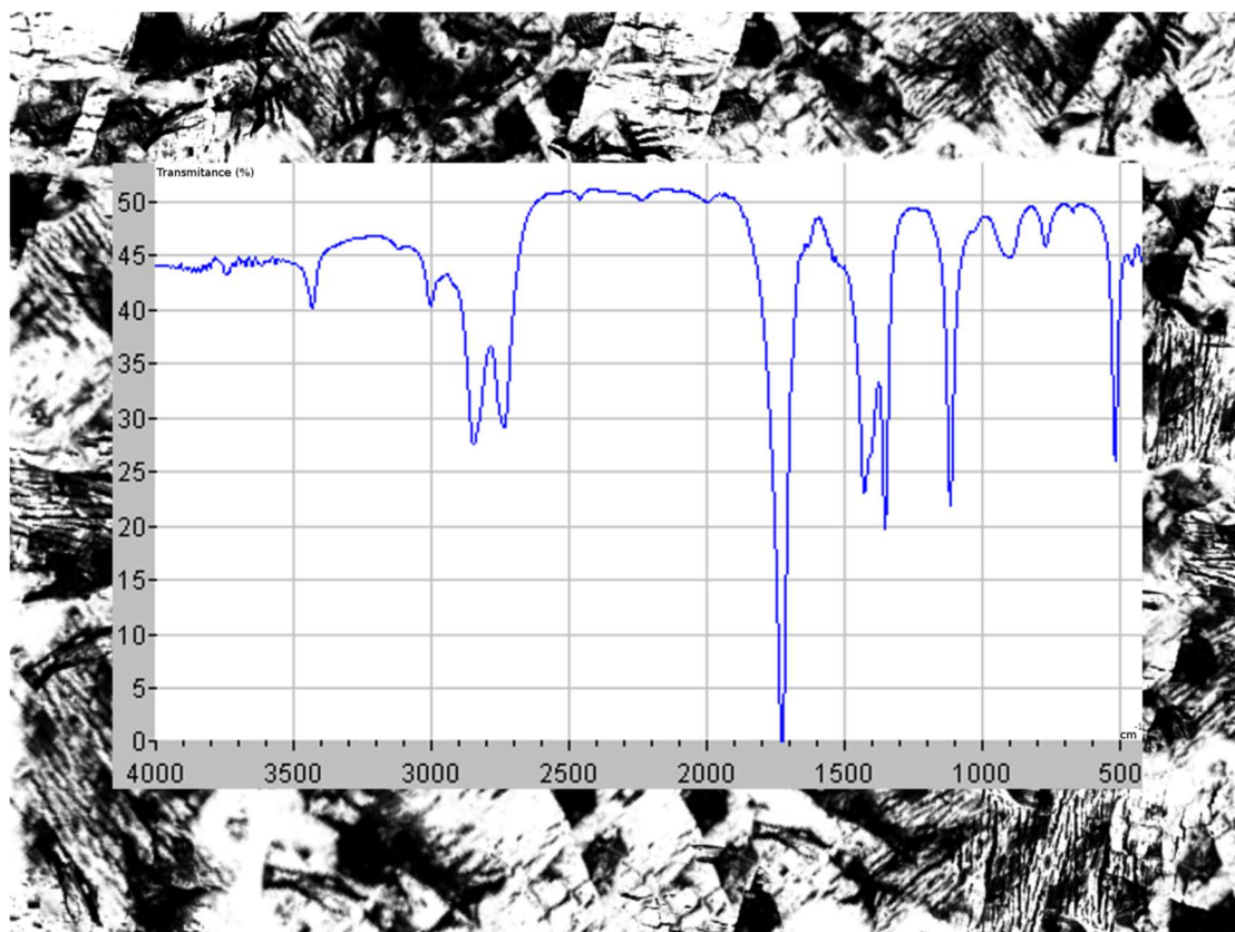
Spectre 1 : \text{C}_2\text{H}_4\text{O}
