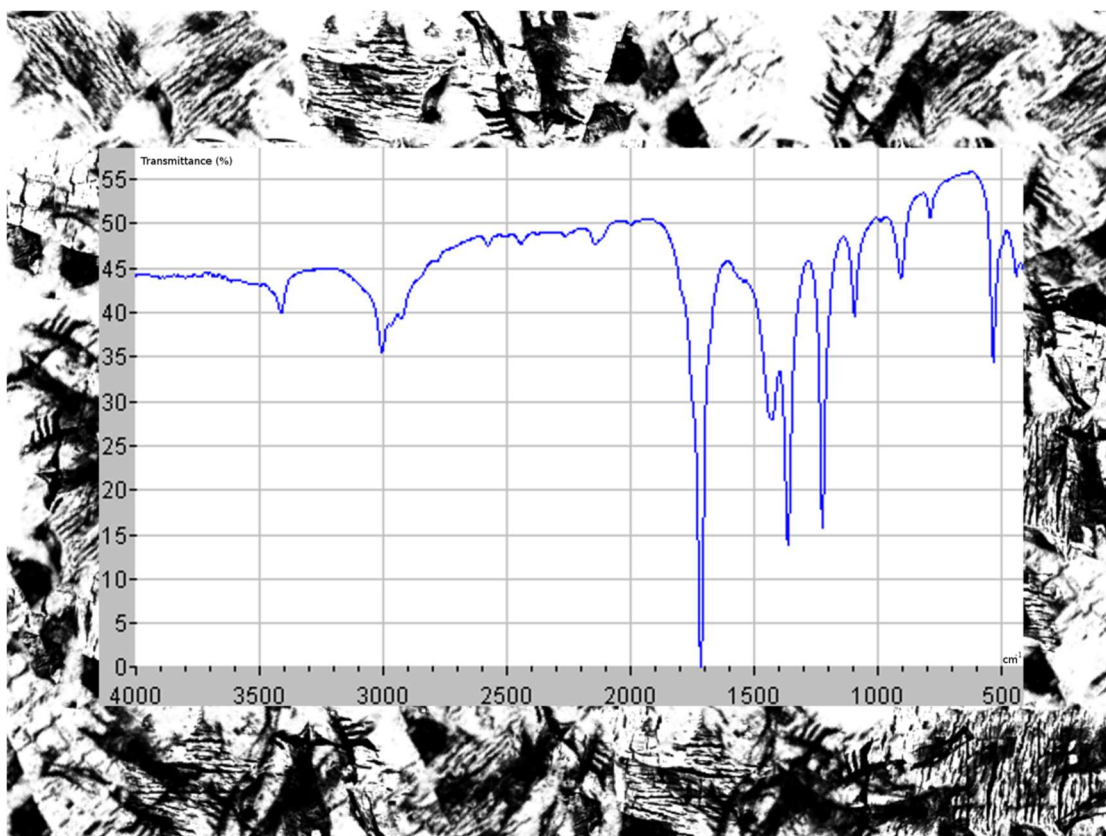
Spectre 3 : C_3H_6O
