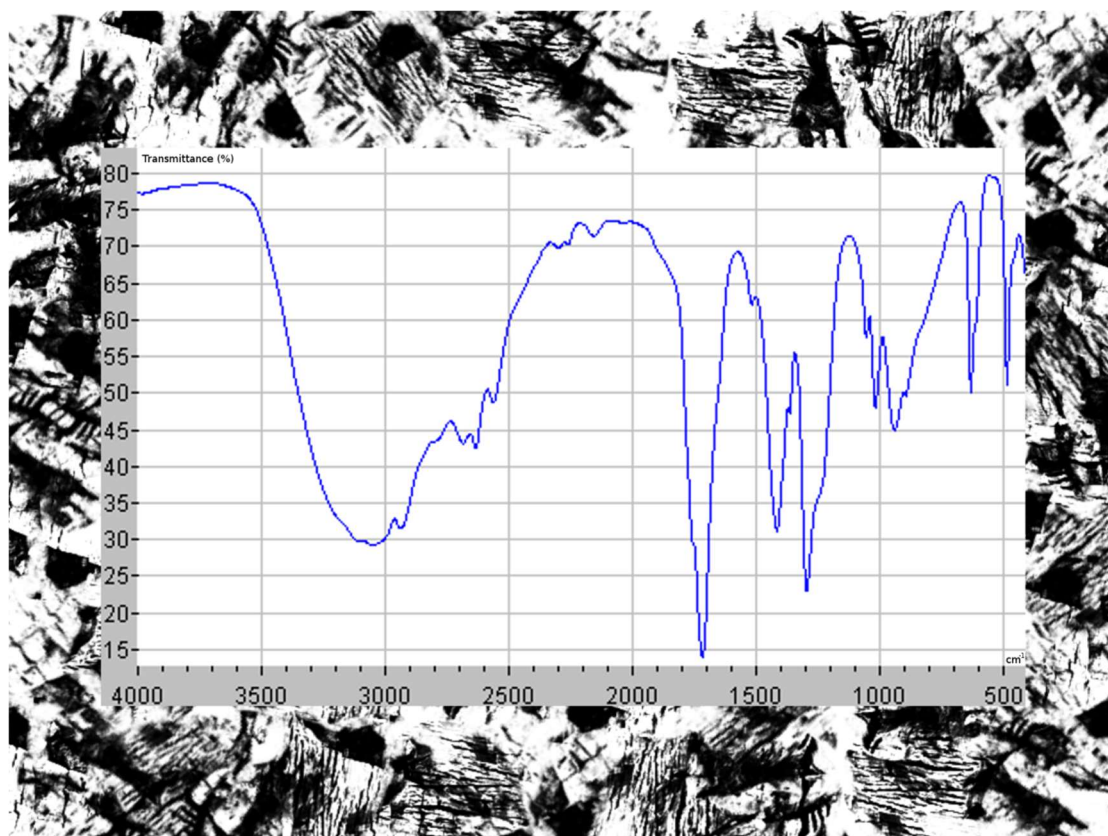
Spectre 4 : \text{C}_2\text{H}_4\text{O}_2
