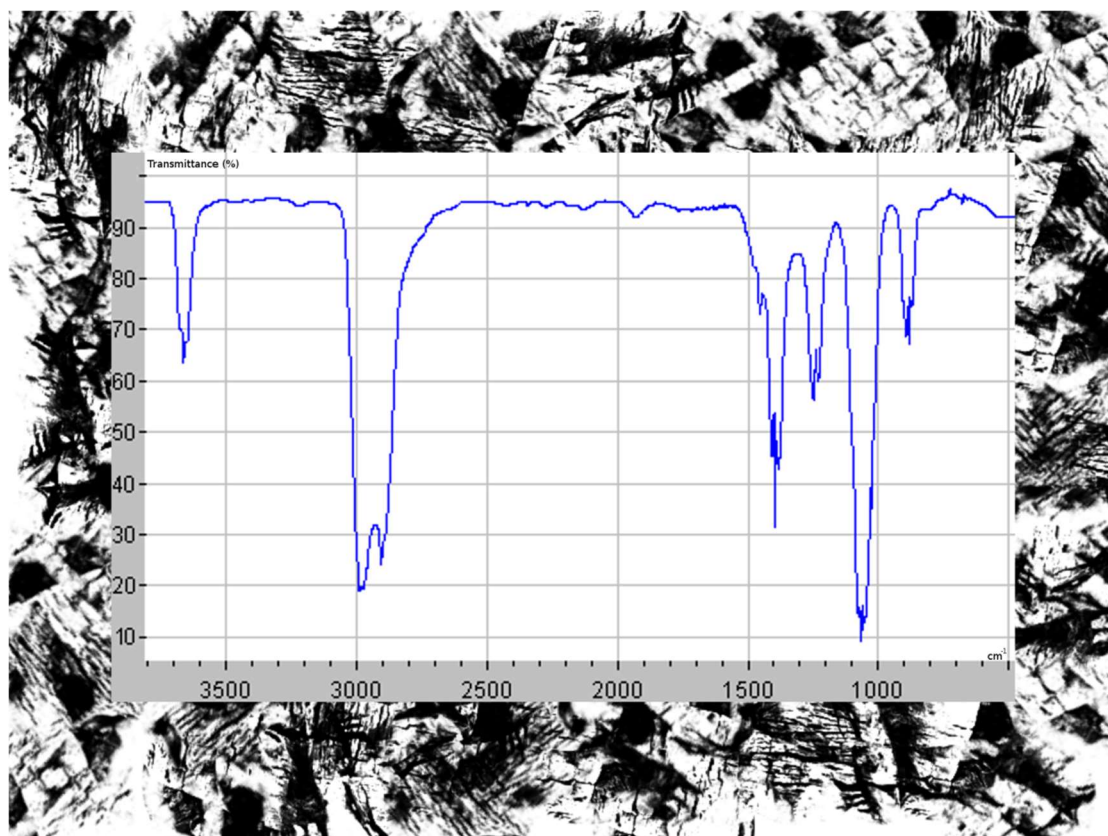
Spectre 6 : \text{C}_2\text{H}_6\text{O}
