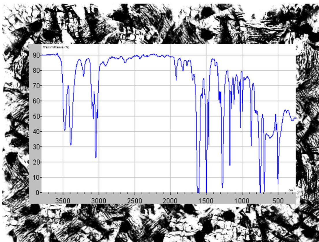
Spectre 5 : C_6H_7N
