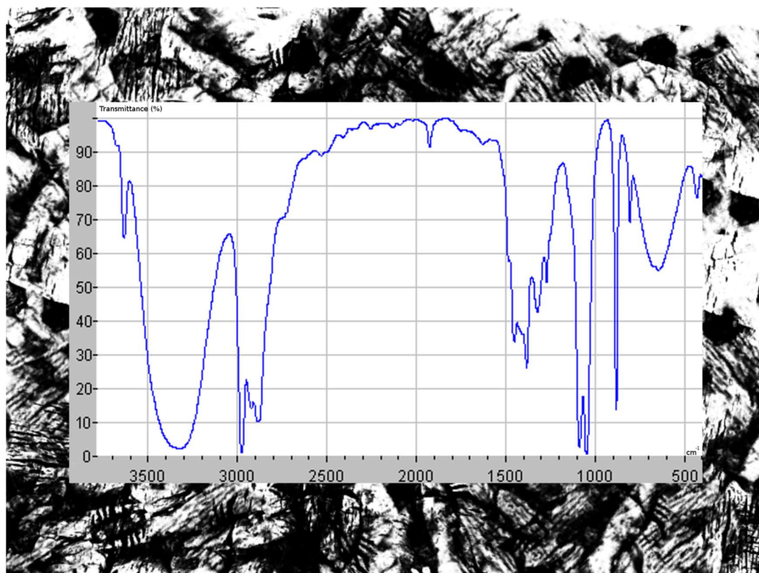
Spectre 7 : \text{C}_2\text{H}_6\text{O}
