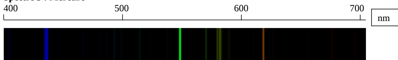
Spectre 6 : Cadmium
